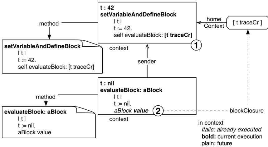
Figure 1.1: Non-local variables are looked in the method activation context where the block was created and not where it is evaluated .
