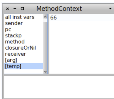
Figure 1.4: A method context where we can access the value of the temporary variable temp at that given point of execution.
