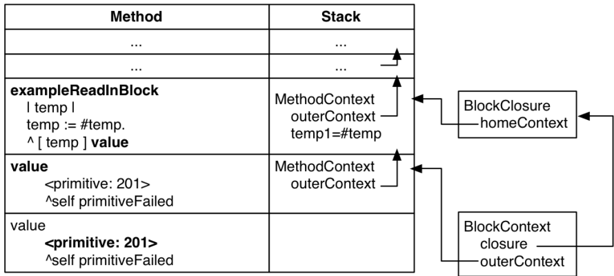
Figure 1.7: A first understanding of closures.
