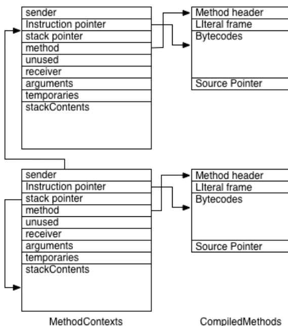
Figure 1.6: Relations between contexts and compiled methods .
