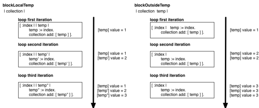
Figure 1.2: blockLocalTemp execution (Left) - blockOutsideTemp execution (Right)
