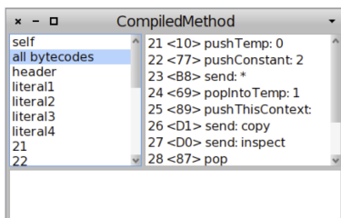
Figure 1.5: The pc variable holds 27 because the last (bytecode) instruction executed was the message send inspect .
