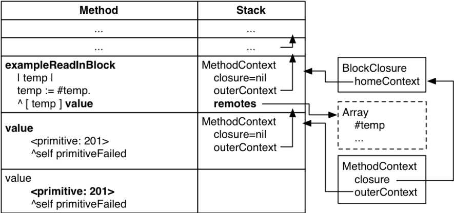
Figure 1.8: How the VM stores remote variables so that they continue to leave when a method returns.
