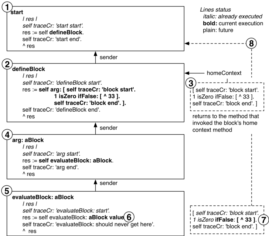
Figure 1.3: A block with non-local return execution returns to the method execution that activated the block home context. Frames represent contexts and dashed frames represent the same block at different execution time.
