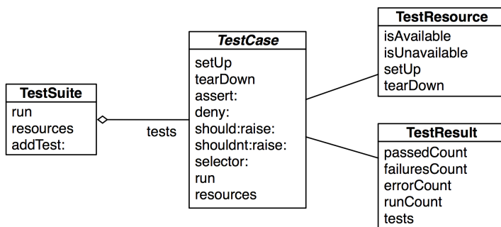
Figure 1.3: The four classes representing the core of SUnit.
