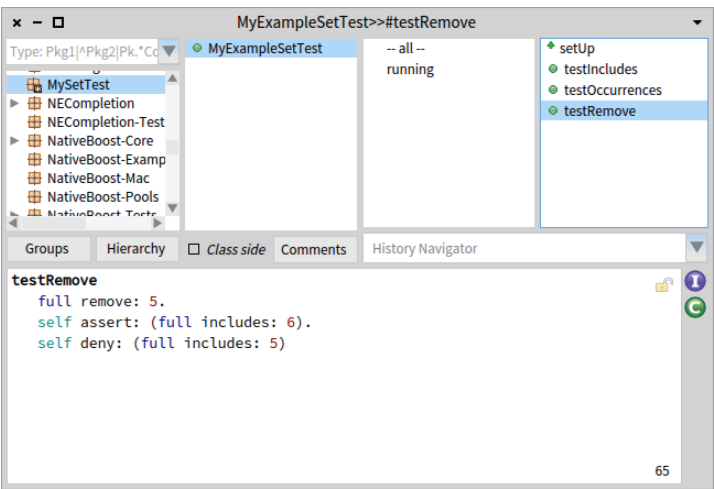
Figure 1.1: Running SUnit tests from the browser.
