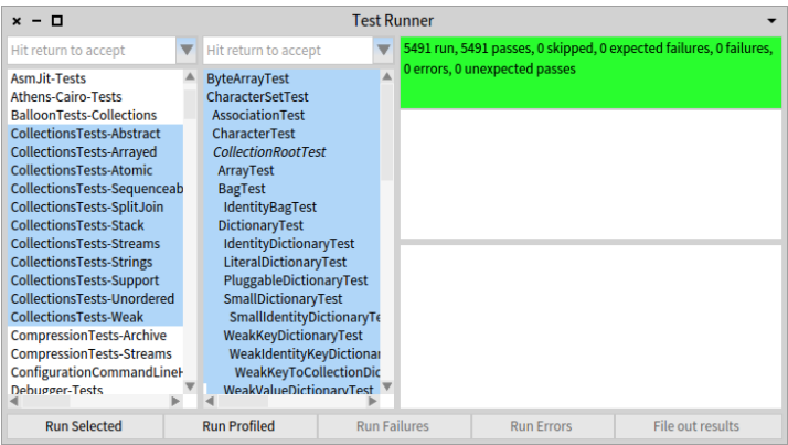
Figure 1.2: Running SUnit tests from the browser.
