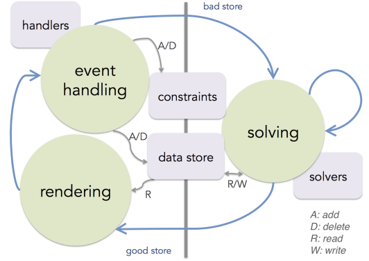
Figure 8. Two-phase execution model in CDP
