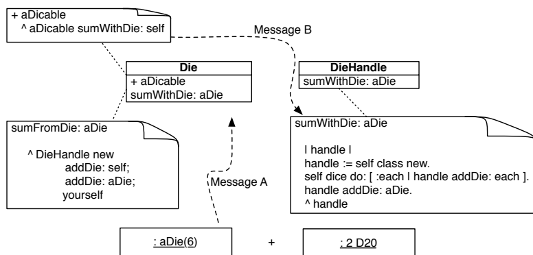
Figure 2.2 Summing a die and a dicable.
