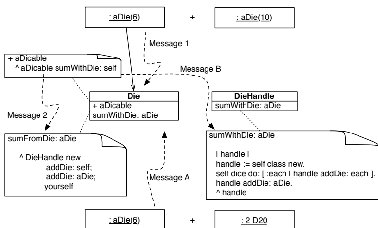
Figure 2.3 Summing a die and a dicable
